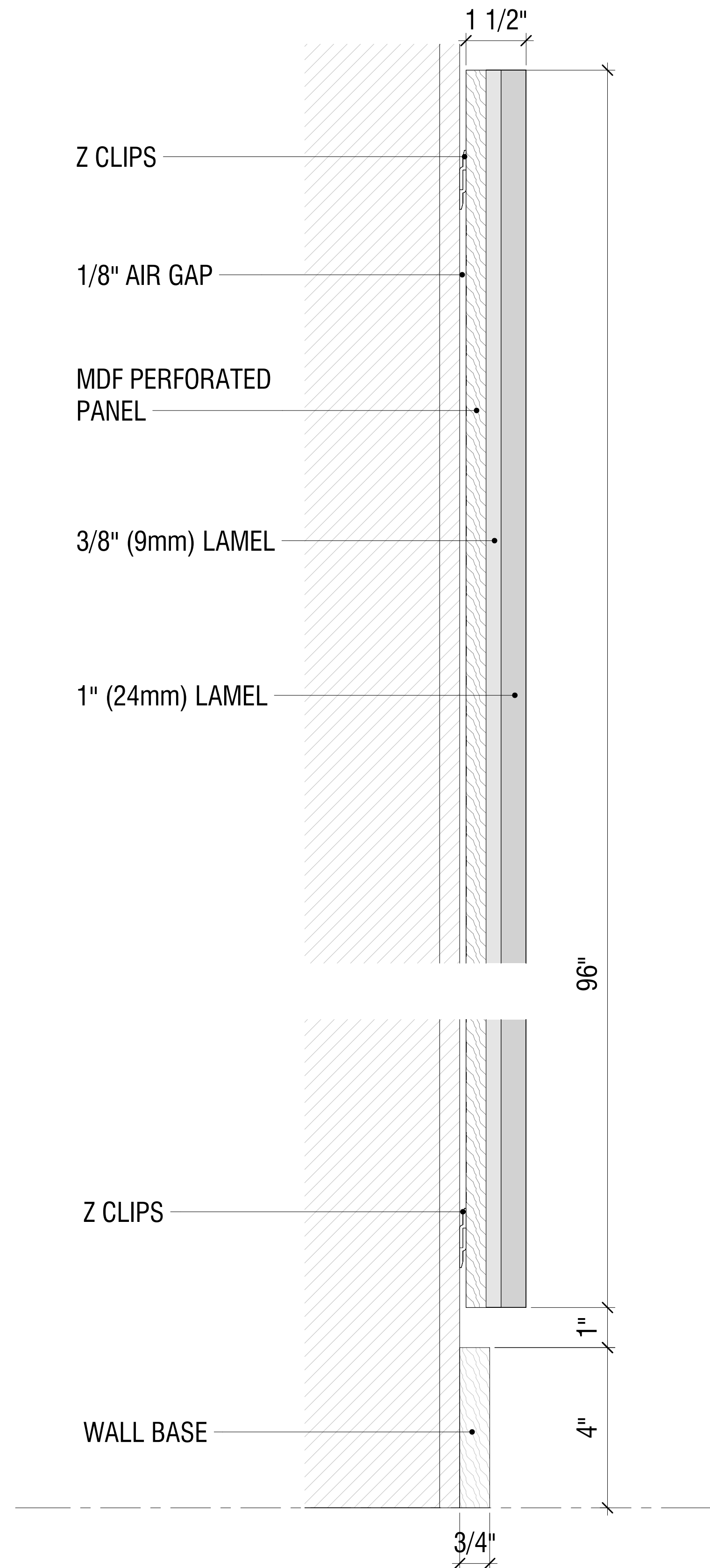
TOCKKY LAMEL MULTI LAYER FELT VERTICAL STAND ALONE PANEL - 4'x8' - SECTIONAL DETAIL ④ 6" = 1'-0"
