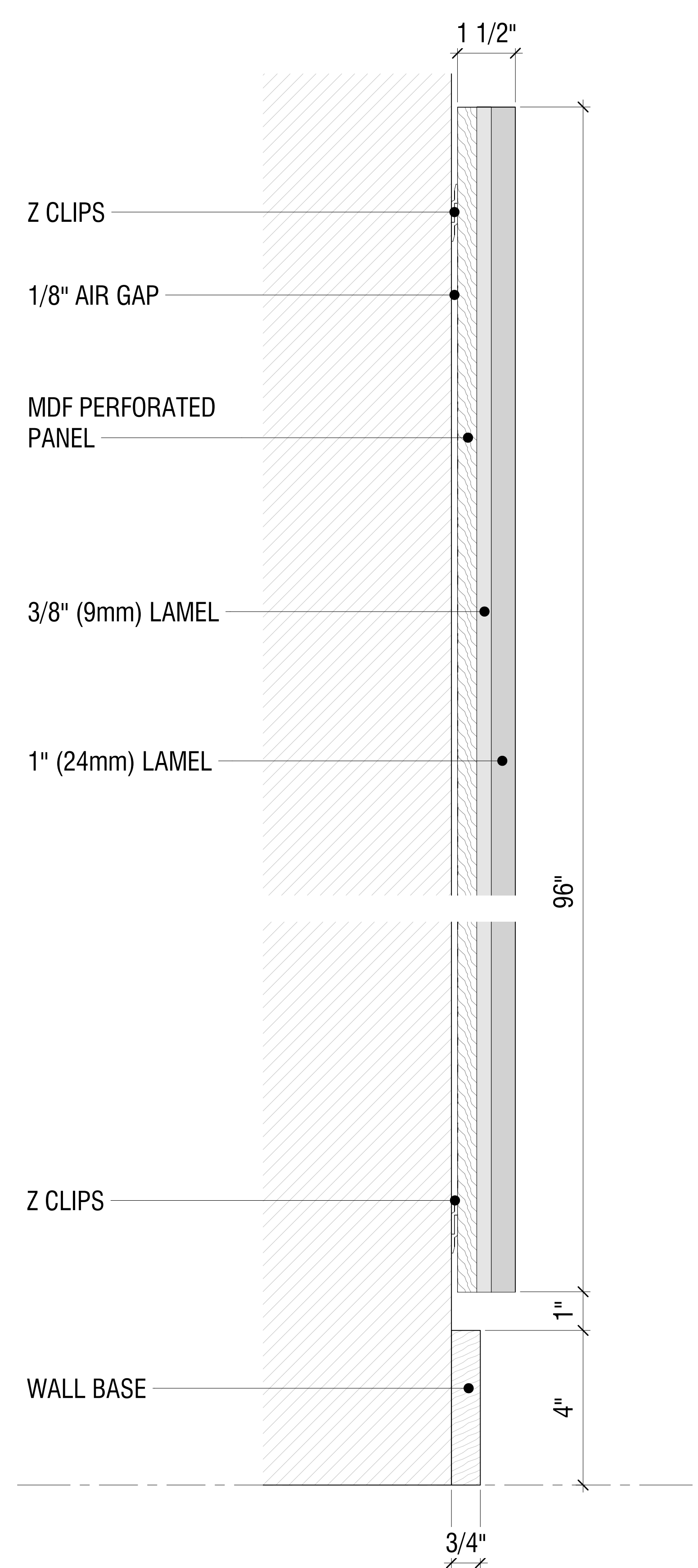
TOCKKY LAMEL MULTI LAYER FELT VERTICAL CONTINUOUS PANEL - 2'x8' - SECTIONAL DETAIL ④ 6" = 1'-0"
