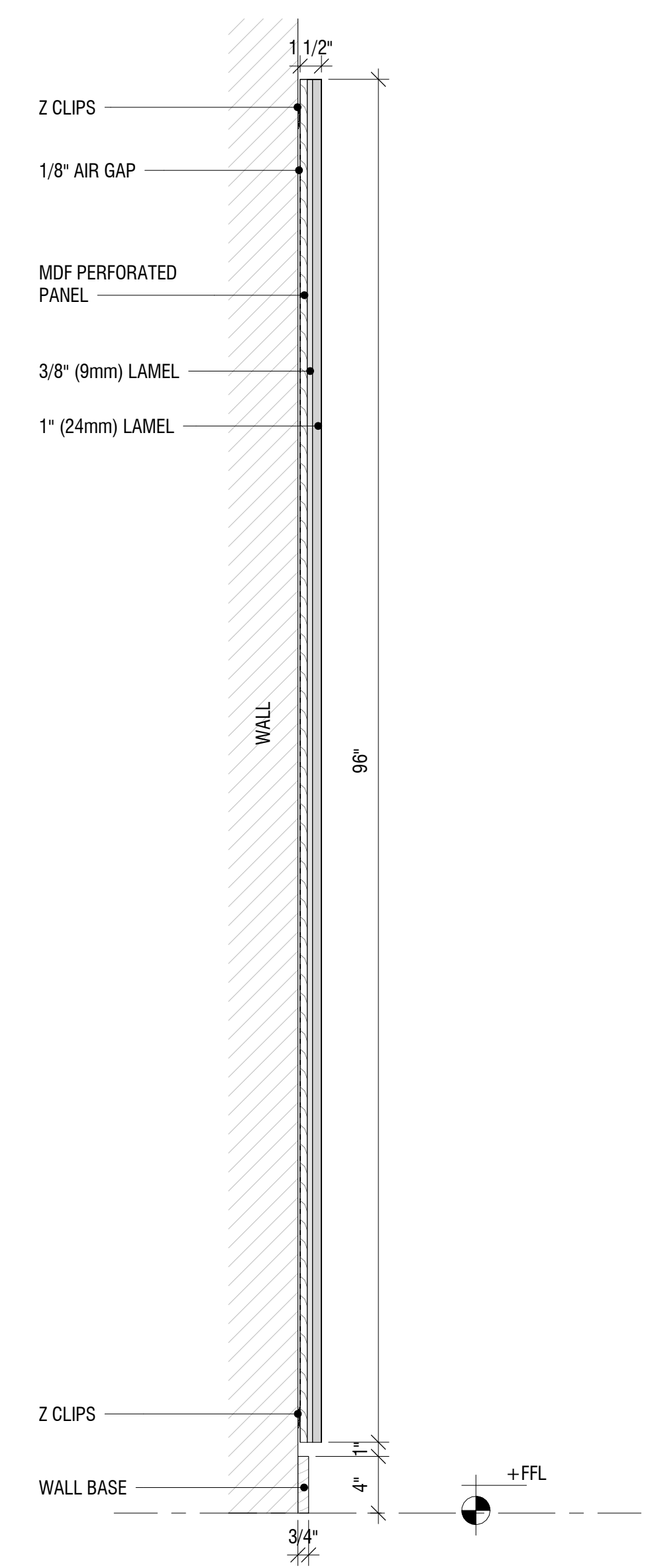
TOCKKY LAMEL MULTI LAYER FELT VERTICAL CONTINUOUS PANEL - 2'x8' - TYP. SECTION ③ 1 1/2" = 1'-0"
