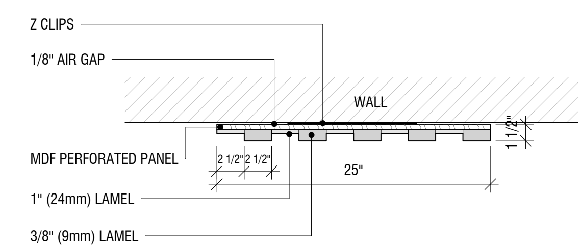
TOCKKY LAMEL MULTI LAYER FELT VERTICAL CONTINUOUS PANEL - 2'x8' - PLAN VIEW ① 1 1/2" = 1'-0"
