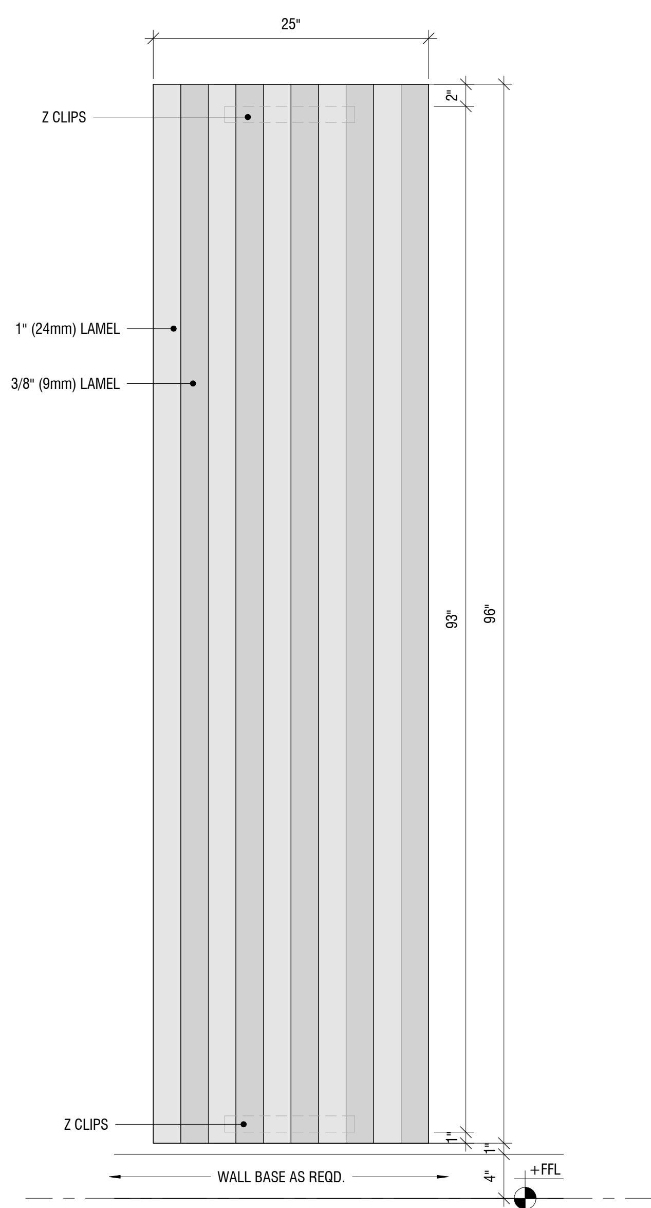
TOCKKY LAMEL MULTI LAYER FELT VERTICAL CONTINUOUS PANEL - 2'x8' - ELEVATION ② 1 1/2" = 1'-0"
