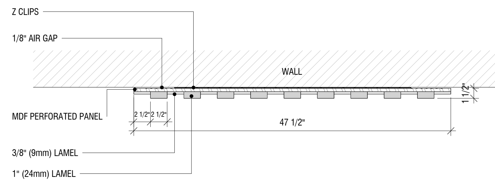
TOCKKY LAMEL MULTI LAYER FELT HORIZONTAL STAND ALONE PANEL - ① 4'x2' - PLAN VIEW 1 1/2" = 1'-0"
