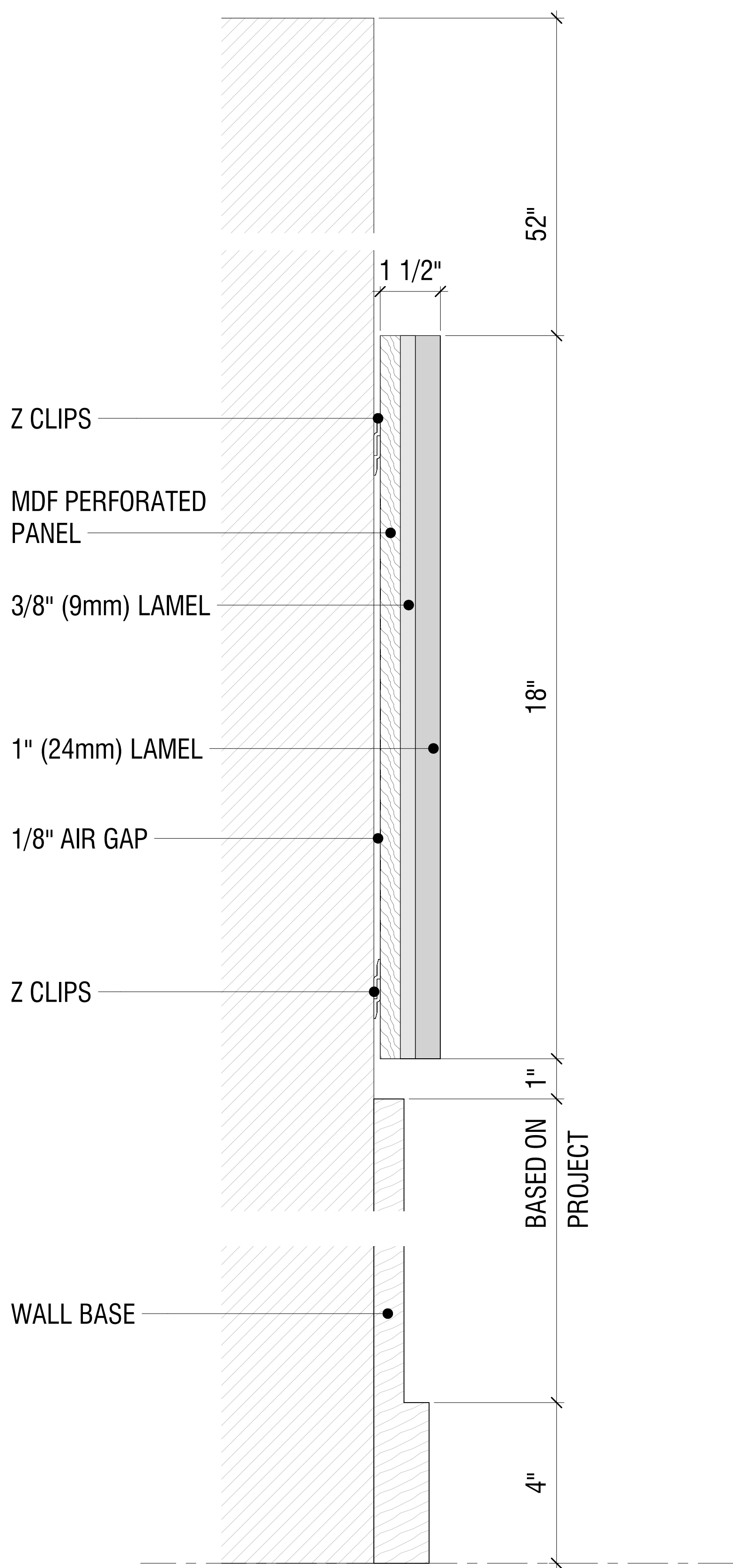
TOCKKY LAMEL MULTI LAYER FELT HORIZONTAL STAND ALONE PANEL - ④ 4'x1 1/2' - SECTIONAL DETAIL 6" = 1'-0"
