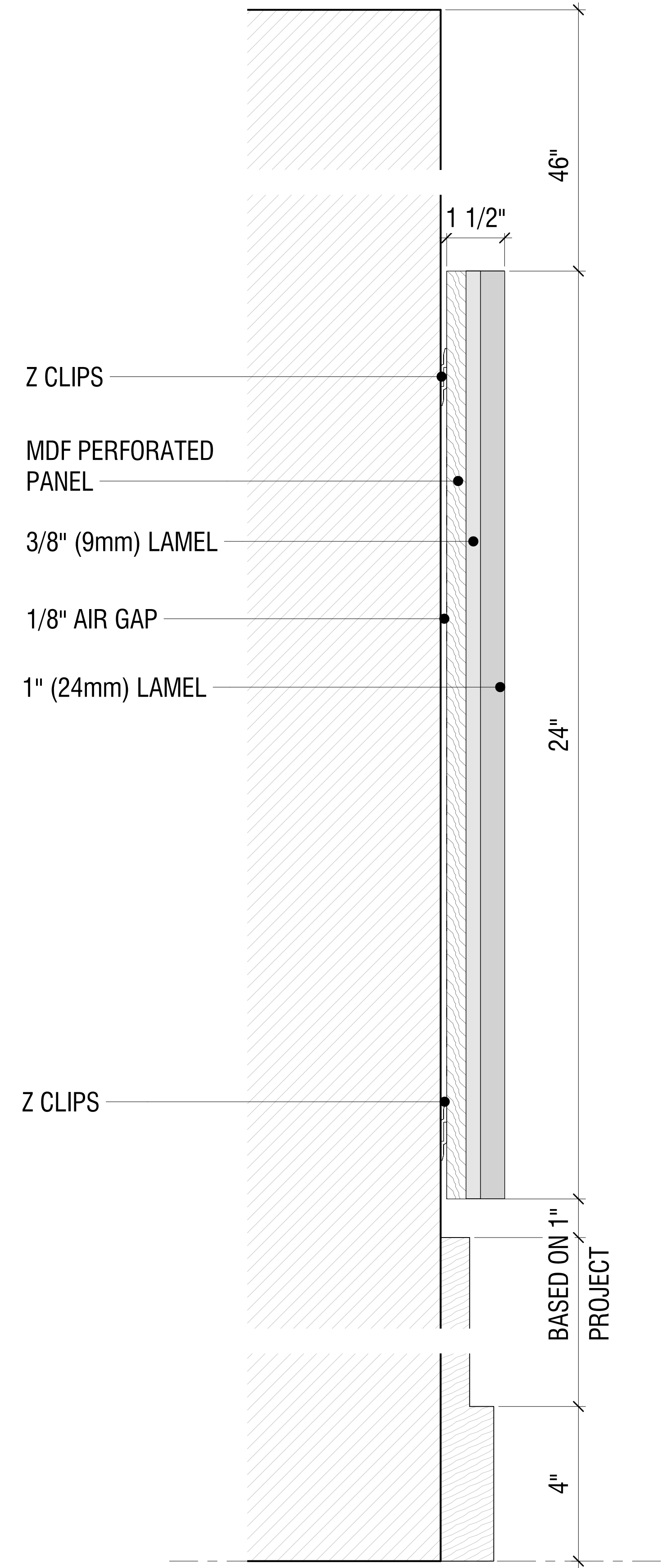
TOCKKY LAMEL MULTI LAYER FELT HORIZONTAL STAND ALONE PANEL - 4'x2' - SECTIONAL DETAIL ④ 6" = 1'-0"
