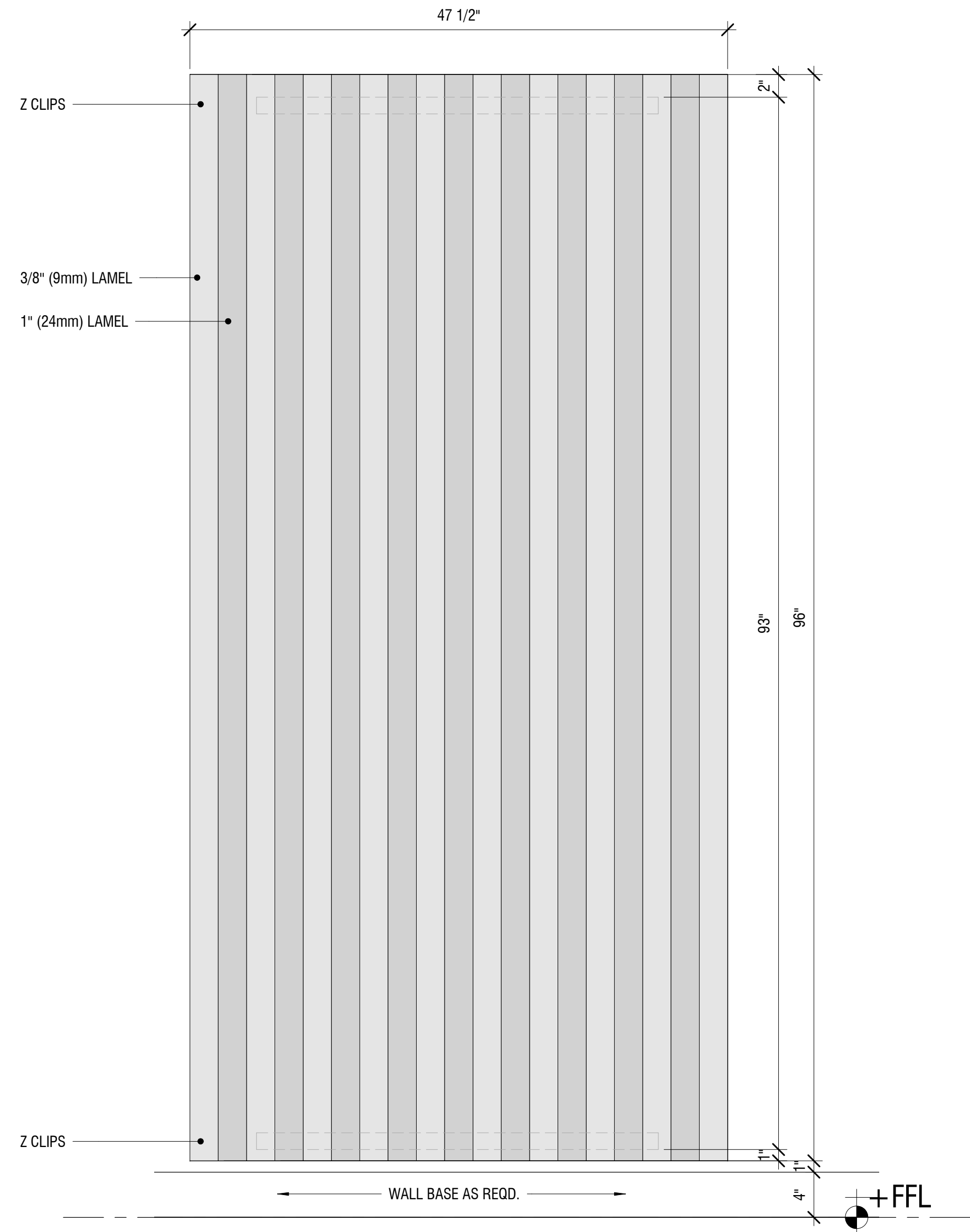
TOCKKY LAMEL MULTI LAYER FELT VERTICAL STAND ALONE PANEL - 4'x8' - ELEVATION ② 1 1/2" = 1'-0"
