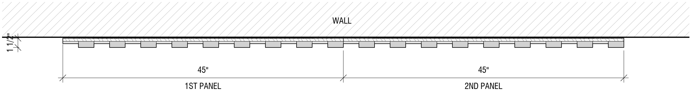
TOCKKY LAMEL MULTI LAYER FELT CONTINUOUS HORIZONTAL PANELS ASSEMBLY 4'x2' - PLAN VIEW 1 1/2" = 1'-0"
