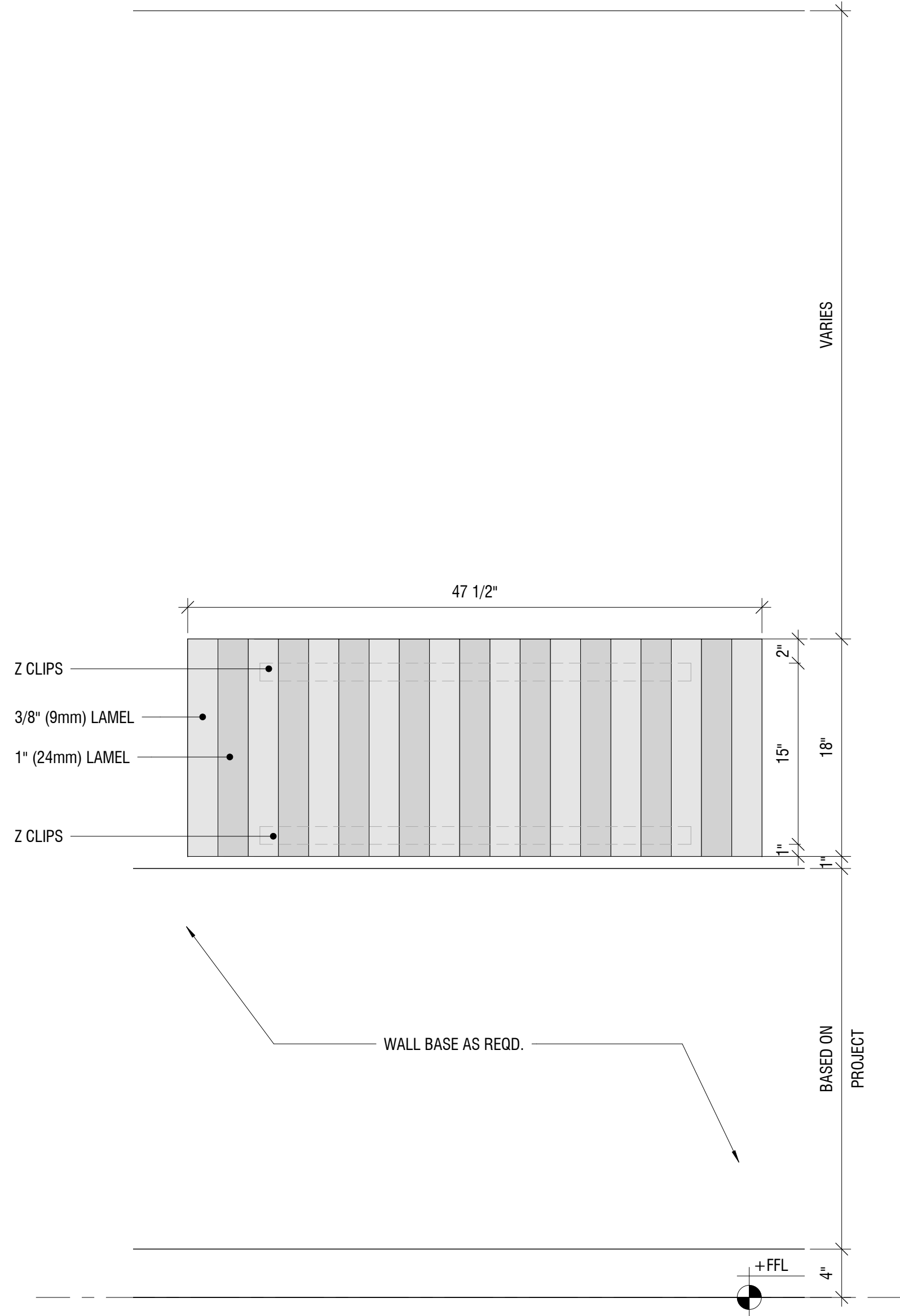
TOCKKY LAMEL MULTI LAYER FELT HORIZONTAL STAND ALONE PANEL - ② 4'x1 1/2' - ELEVATION 1 1/2" = 1'-0"
