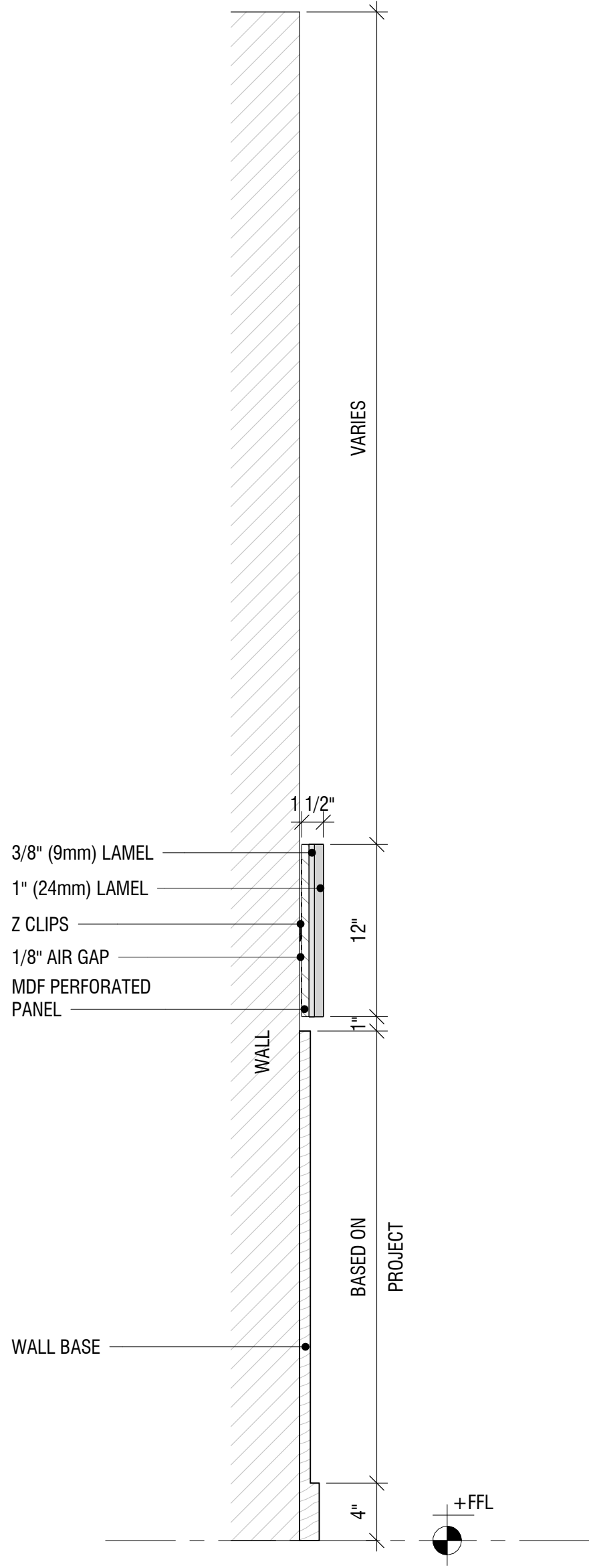
TOCKKY LAMEL MULTI LAYER FELT HORIZONTAL STAND ALONE PANEL - ③ 4'x1' - TYP. SECTION 1 1/2" = 1'-0"
