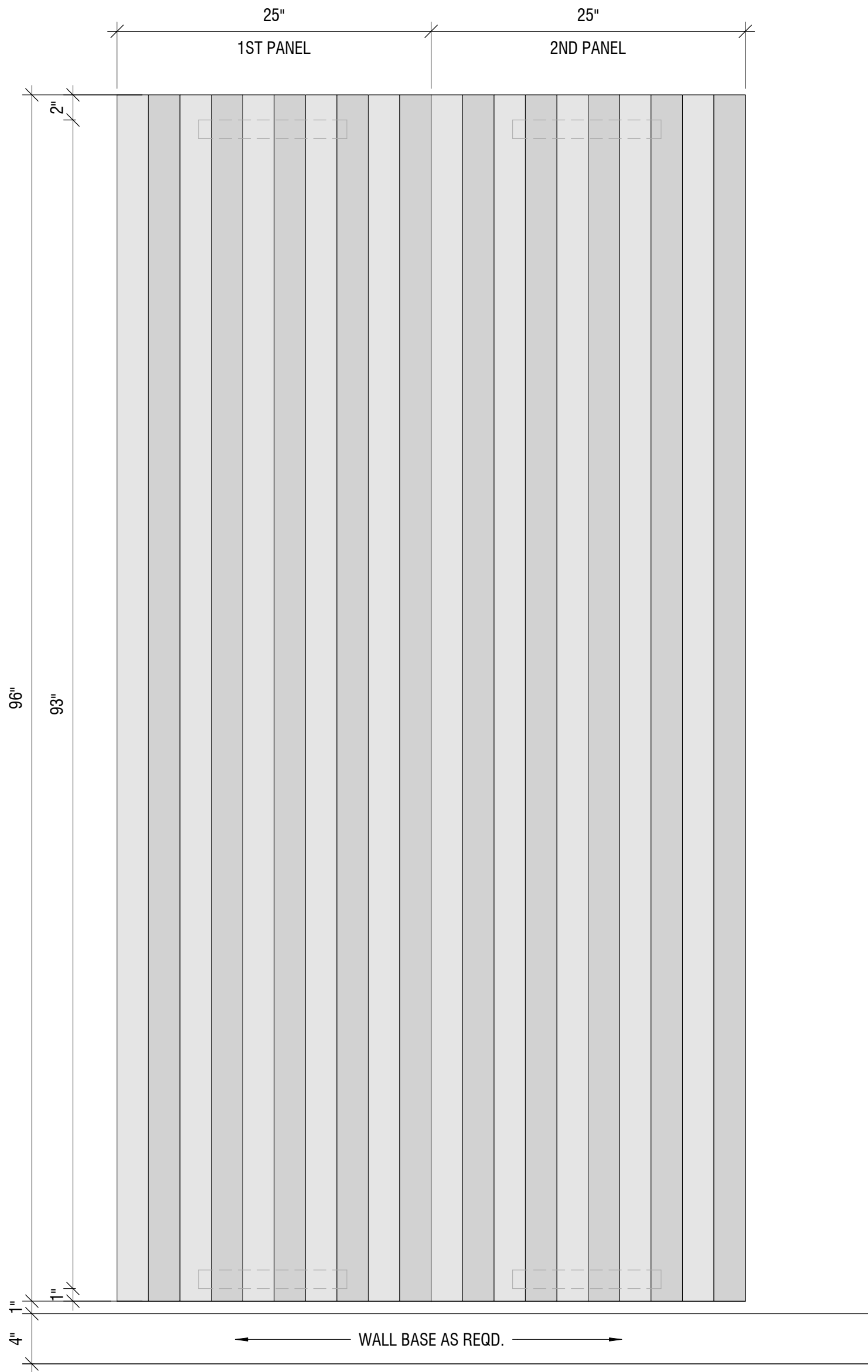
TOCKKY LAMEL MULTI LAYER FELT CONTINUOUS VERTICAL PANELS ASSEMBLY 2'x8' - ELEVATION ② 1 1/2" = 1'-0"
