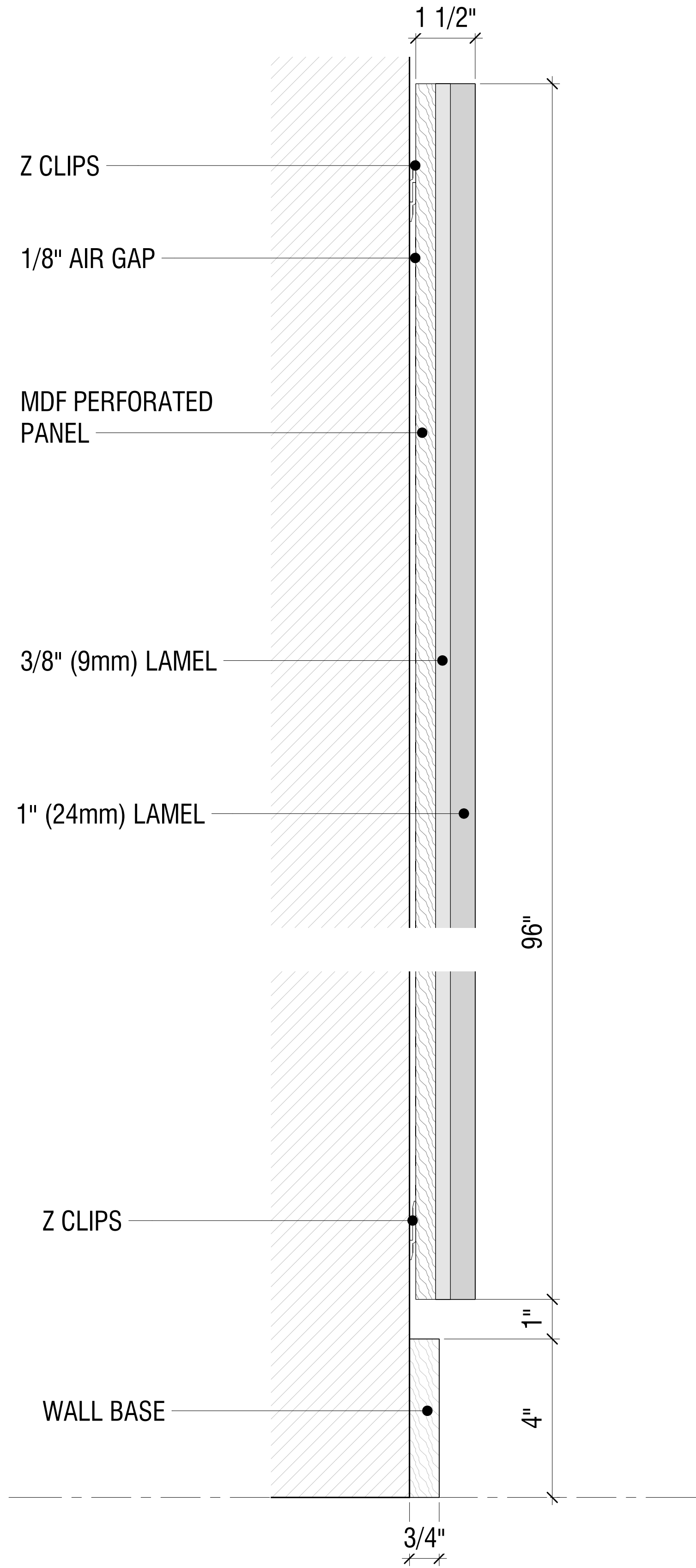
④ TOCKKY LAMEL MULTI LAYER FELT VERTICAL STAND ALONE PANEL - 2'x8' - SECTIONAL DETAIL 6" = 1'-0"
