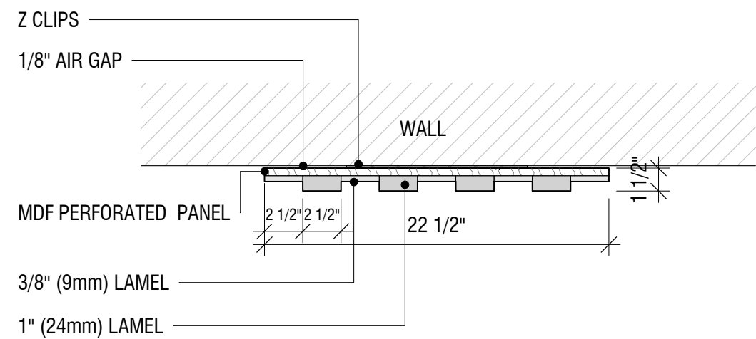
① TOCKKY LAMEL MULTI LAYER FELT VERTICAL STAND ALONE PANEL - 2'x8' - PLAN VIEW 1 1/2" = 1'-0"
