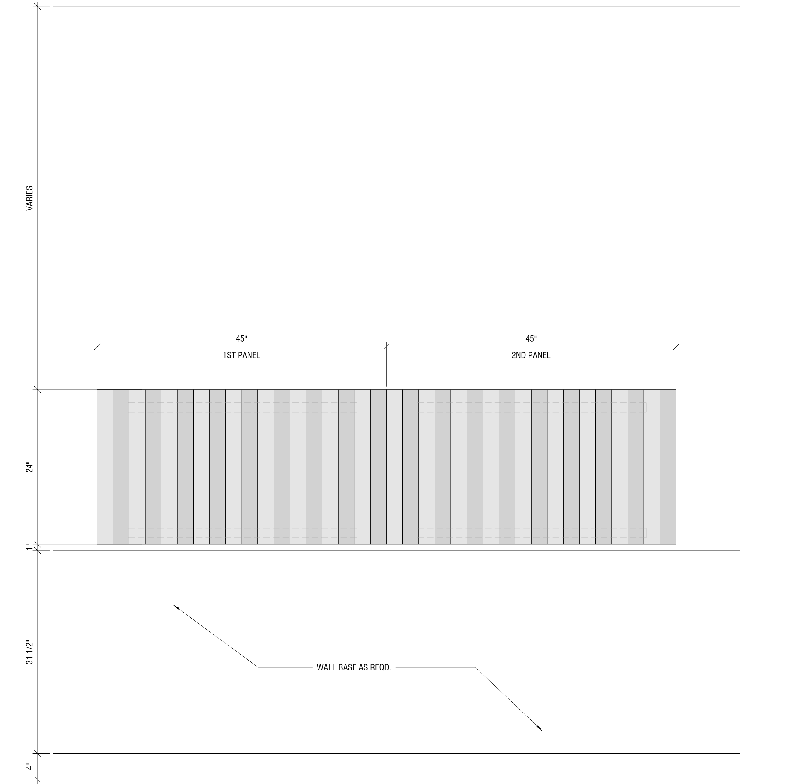
TOCKKY LAMEL MULTI LAYER FELT CONTINUOUS HORIZONTAL PANELS ASSEMBLY 4'x2' - ELEVATION 1 1/2" = 1'-0"
