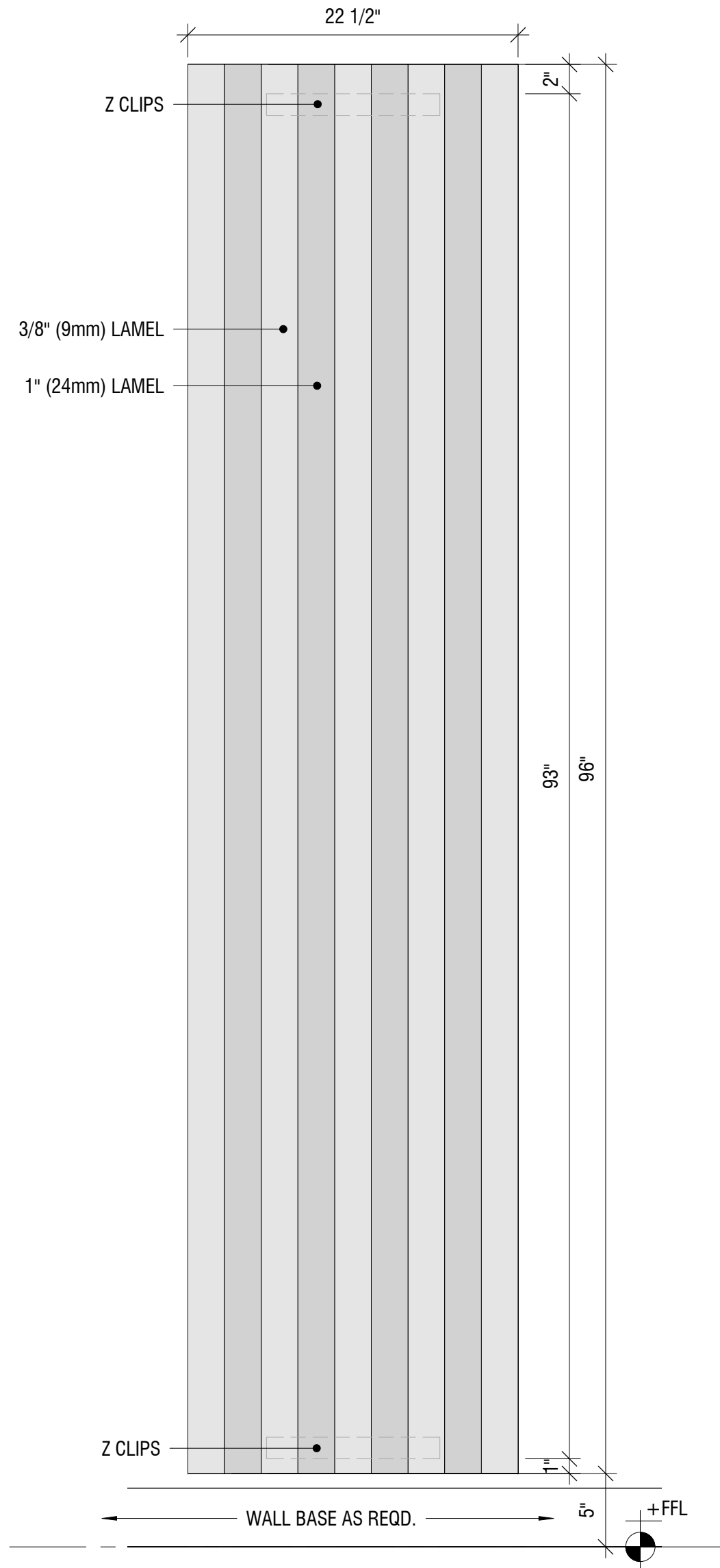
② TOCKKY LAMEL MULTI LAYER FELT VERTICAL STAND ALONE PANEL - 2'x8' - ELEVATION 1 1/2" = 1'-0"
