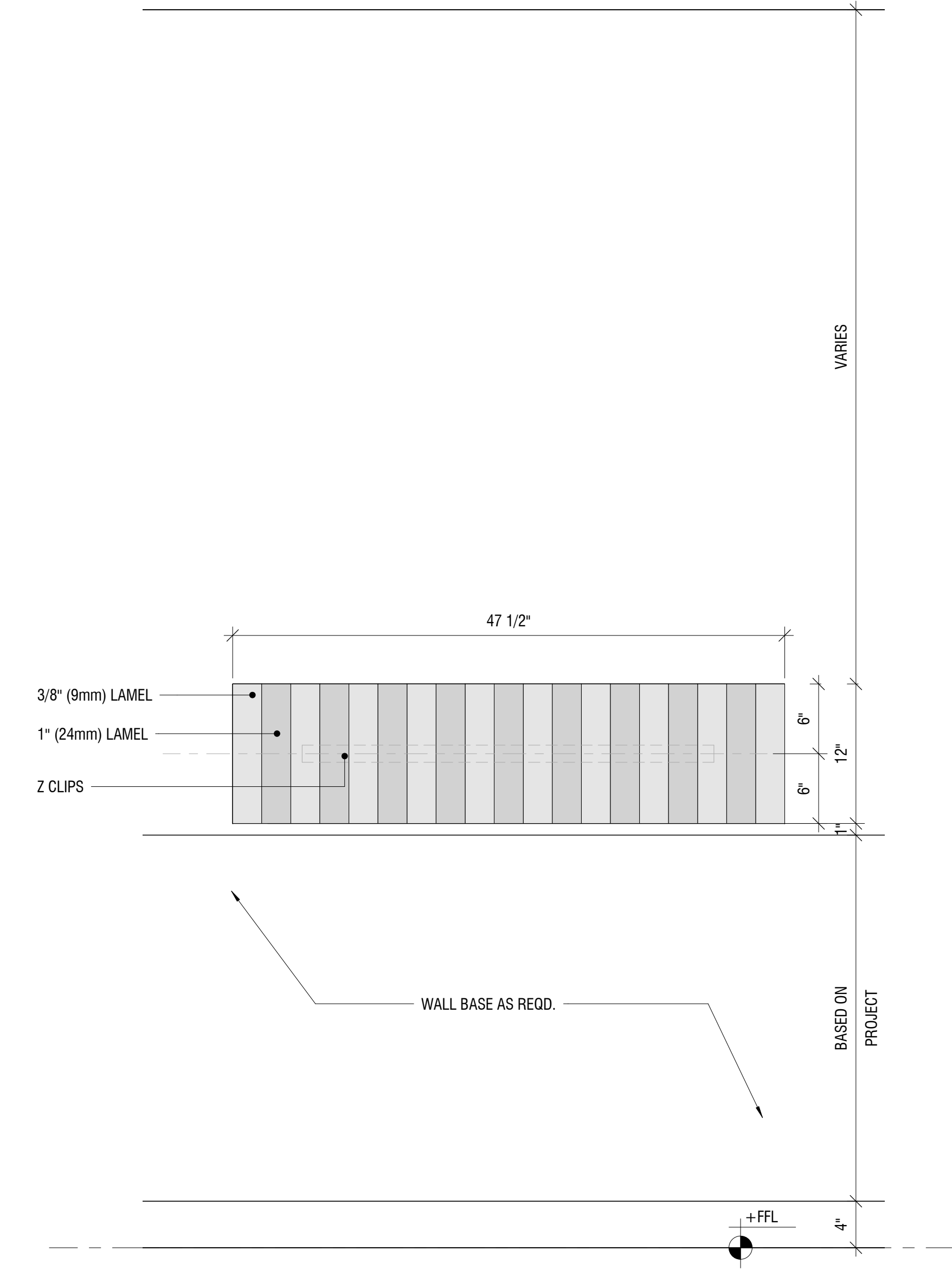
TOCKKY LAMEL MULTI LAYER FELT HORIZONTAL STAND ALONE PANEL - ② 4'x1' - ELEVATION 1 1/2" = 1'-0"
