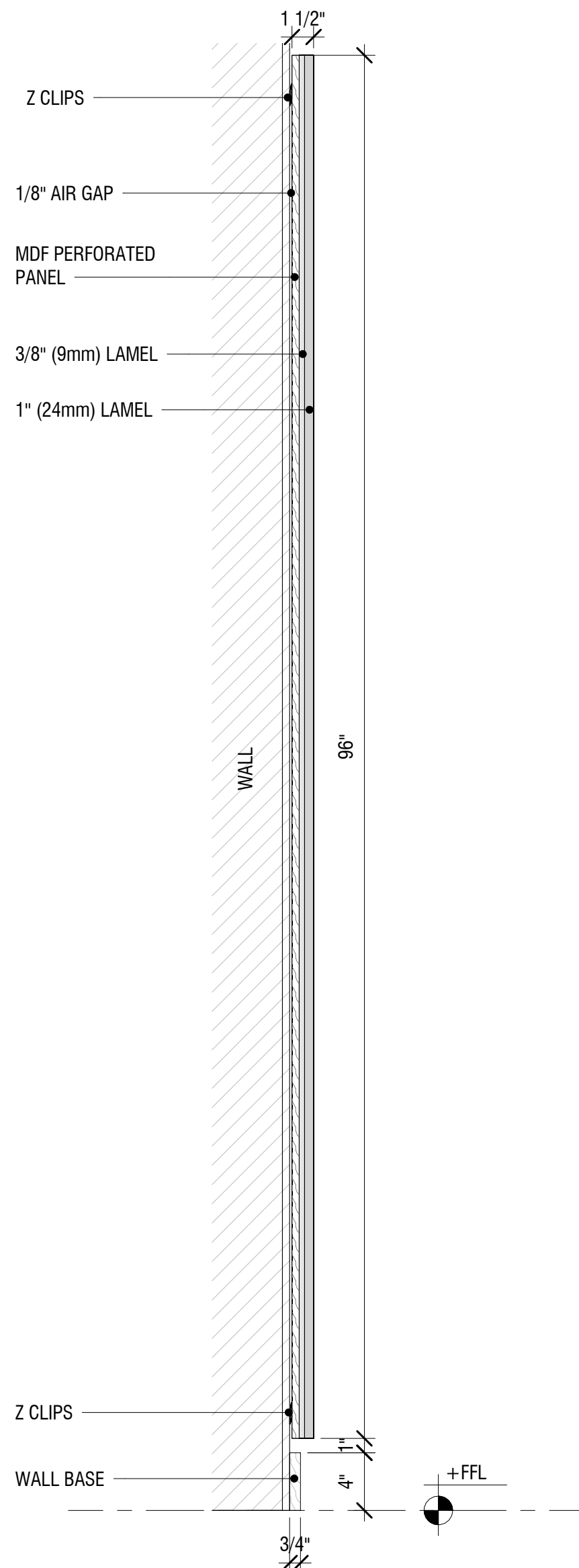
TOCKKY LAMEL MULTI LAYER FELT VERTICAL STAND ALONE PANEL - 4'x8' - TYP. SECTION ③ 1 1/2" = 1'-0"
