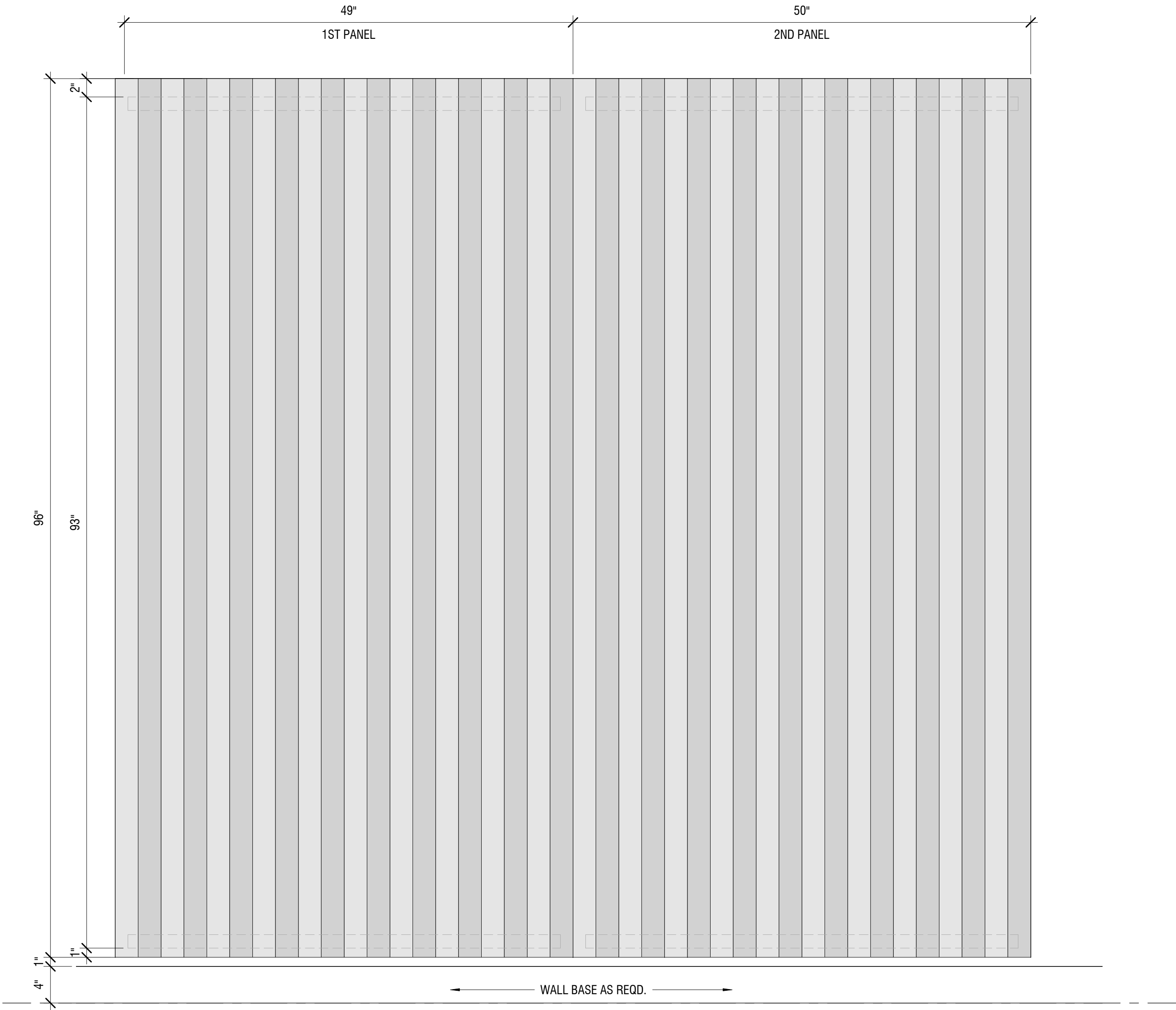
TOCKKY LAMEL MULTI LAYER FELT CONTINUOUS VERTICAL PANELS ASSEMBLY 4'x8' - ELEVATION ② 1 1/2" = 1'-0"
