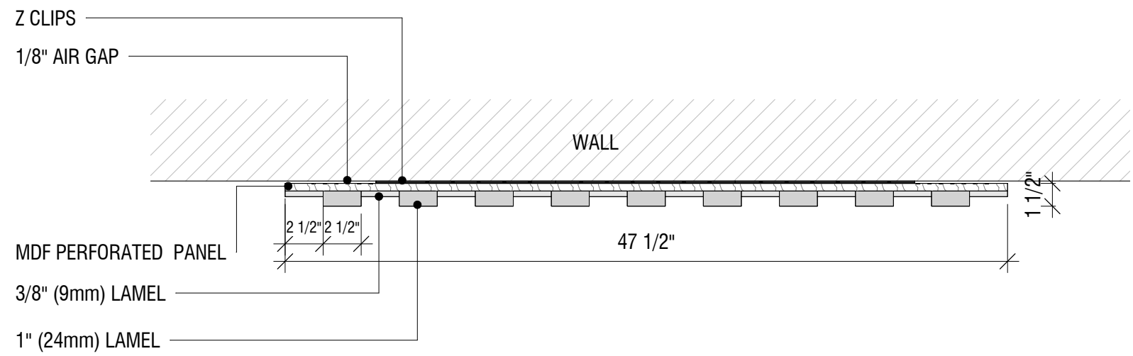
TOCKKY LAMEL MULTI LAYER FELT HORIZONTAL STAND ALONE PANEL - ① 4'x1 1/2' - PLAN VIEW 1 1/2" = 1'-0"
