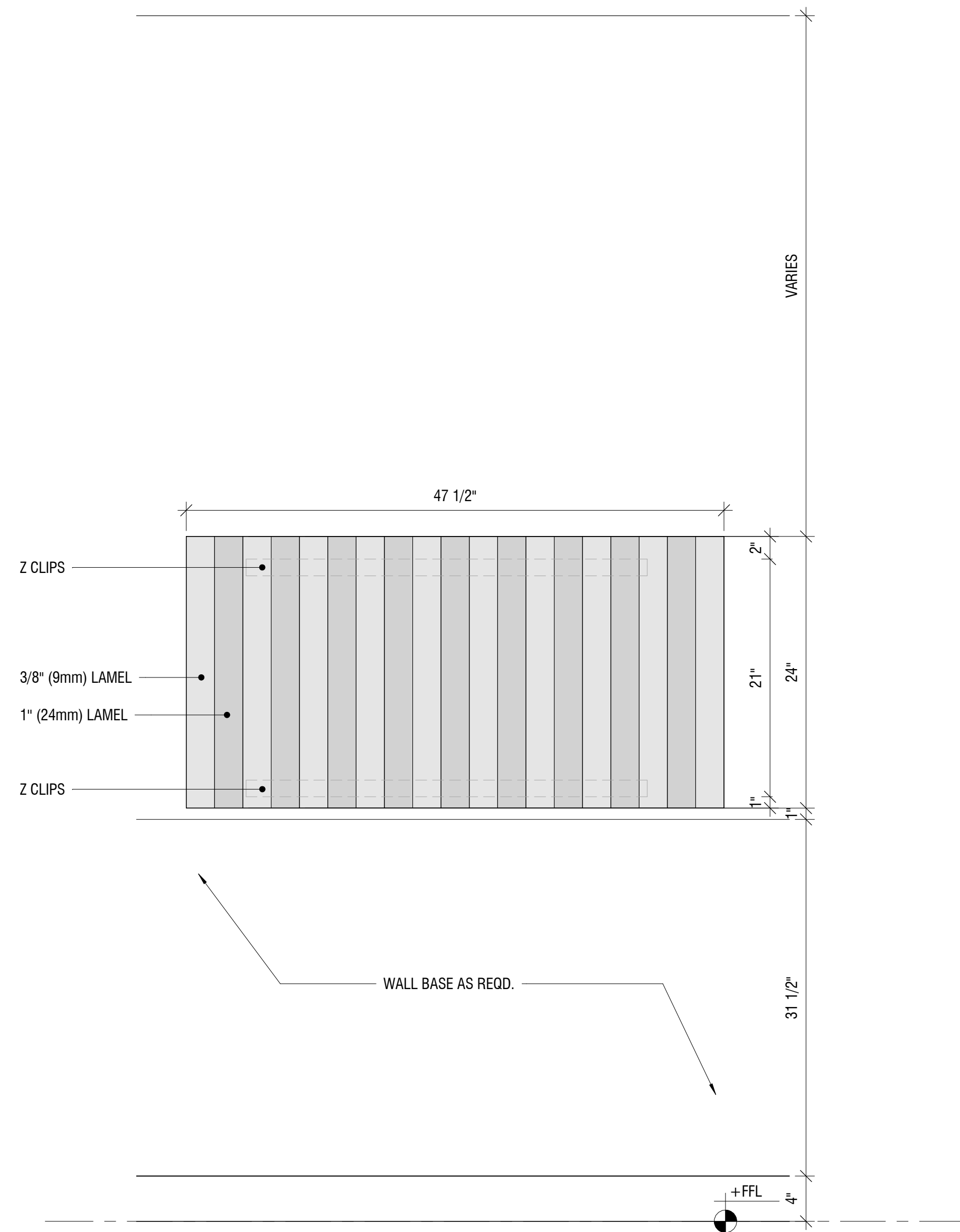
TOCKKY LAMEL MULTI LAYER FELT HORIZONTAL STAND ALONE PANEL - ② 4'x2' - ELEVATION 1 1/2" = 1'-0"
