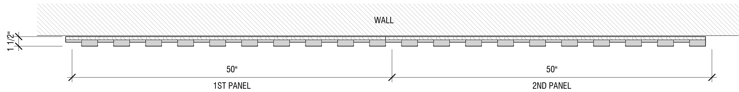
TOCKKY LAMEL MULTI LAYER FELT CONTINUOUS VERTICAL PANELS ASSEMBLY 4'x8' - PLAN VIEW ① 1 1/2" = 1'-0"
