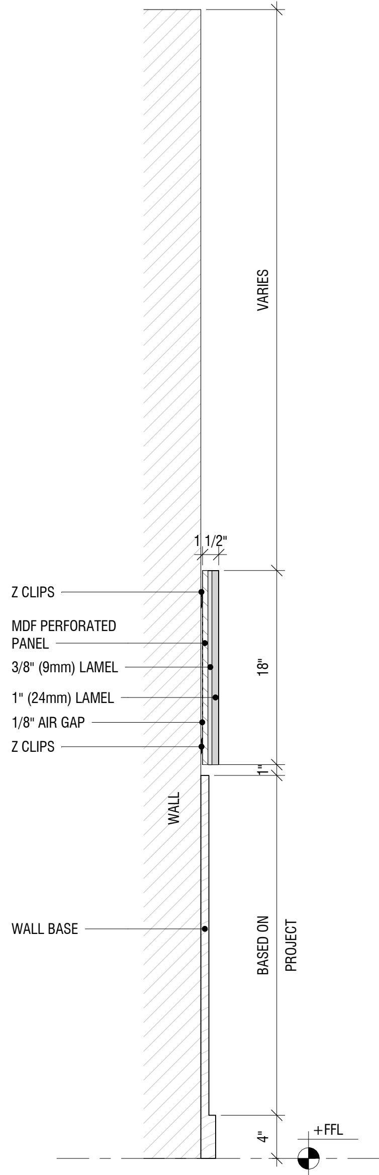
TOCKKY LAMEL MULTI LAYER FELT HORIZONTAL STAND ALONE PANEL - ③ 4'x1 1/2' - TYP. SECTION 1 1/2" = 1'-0"
