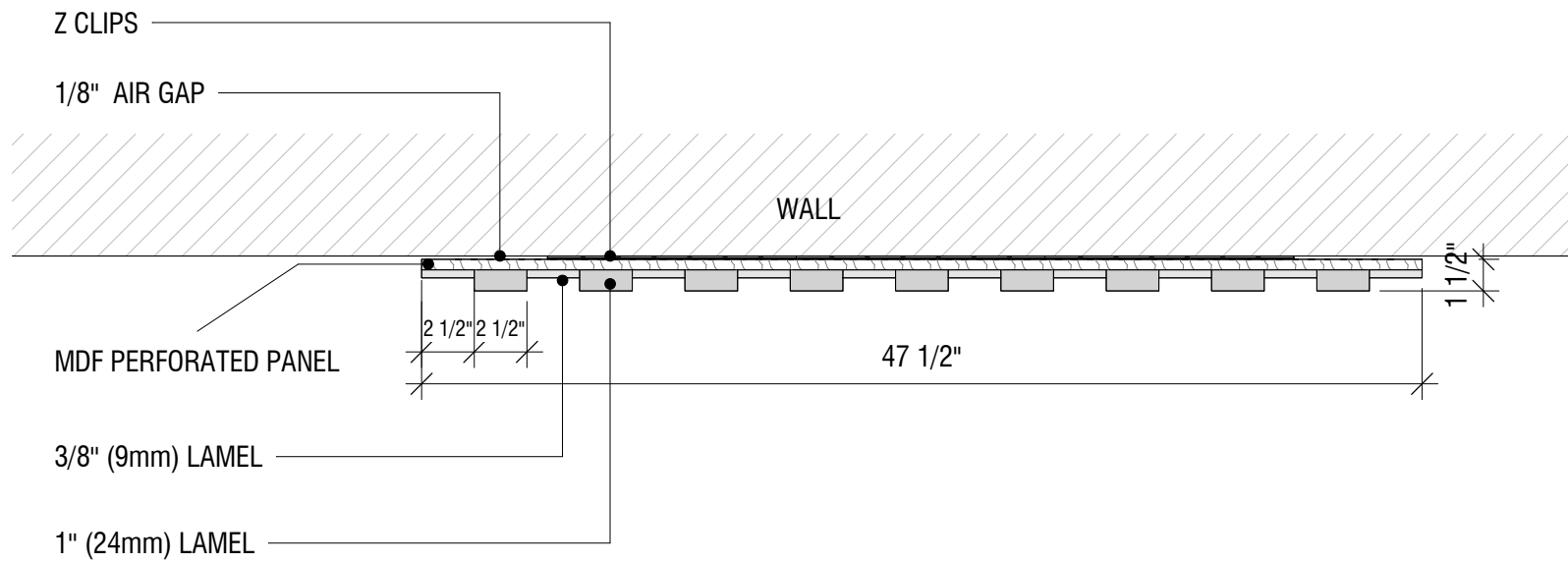
TOCKKY LAMEL MULTI LAYER FELT HORIZONTAL STAND ALONE PANEL - ① 4'x1' - PLAN VIEW 1 1/2" = 1'-0"
