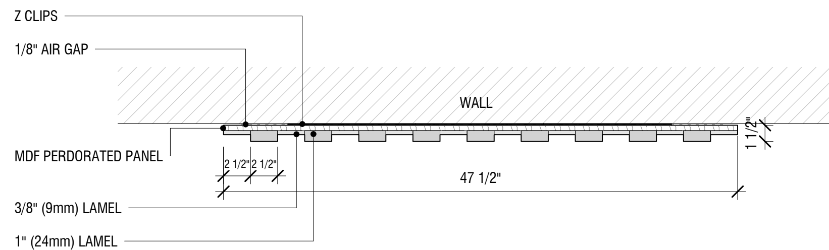
TOCKKY LAMEL MULTI LAYER FELT VERTICAL STAND ALONE PANEL - 4'x8' - PLAN VIEW ① 1 1/2" = 1'-0"
