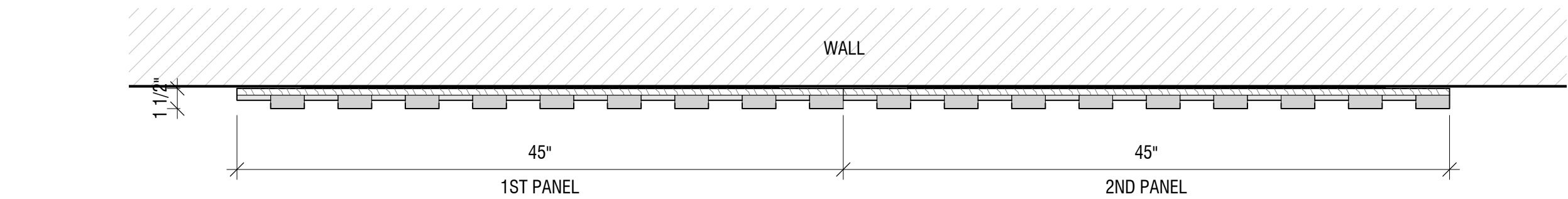
TOCKKY LAMEL MULTI LAYER FELT CONTINUOUS HORIZONTAL PANELS ASSEMBLY 4'x1 1/2' - PLAN VIEW 1 1/2" = 1'-0"
