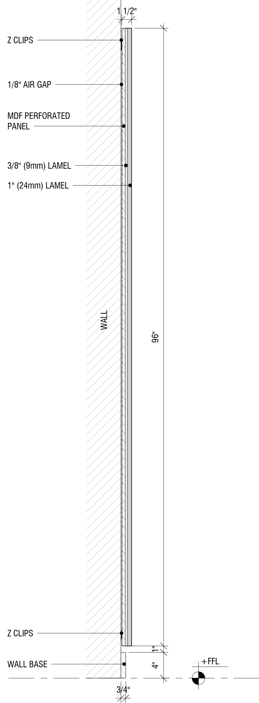
③ TOCKKY LAMEL MULTI LAYER FELT VERTICAL STAND ALONE PANEL - 2'x8' - TYP. SECTION 1 1/2" = 1'-0"
